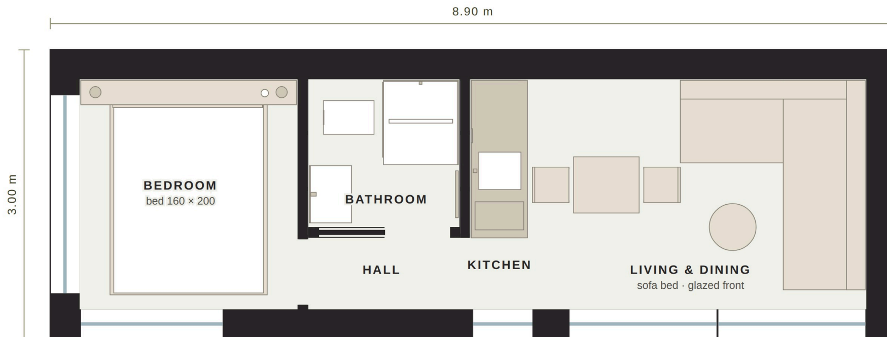
FJORD · 3.00 M WIDE BODY · GLAZED FRONT ON THE LOWER SIDE
